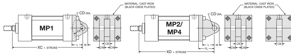
FM Series MP1 & MP2 Clevis and MP4 Rod Eye Mount Dimensions
