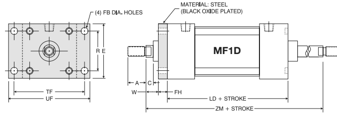
FM Series Double Rod End MF1D Flange Mount Dimensions
