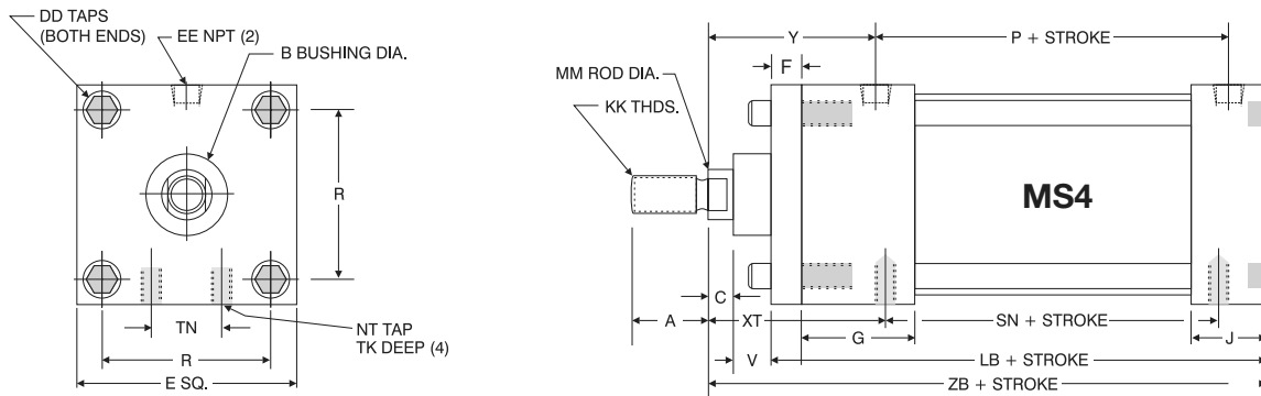
FM Series Oversize Rod MS4 Flush Mount Dimensions
