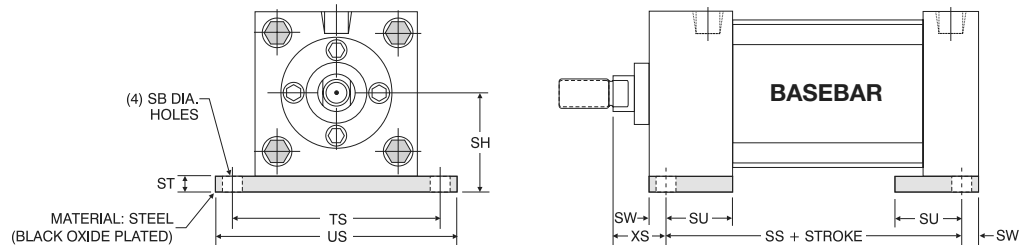
FM Series Basebar Mount (Non-NFPA) Dimensions
