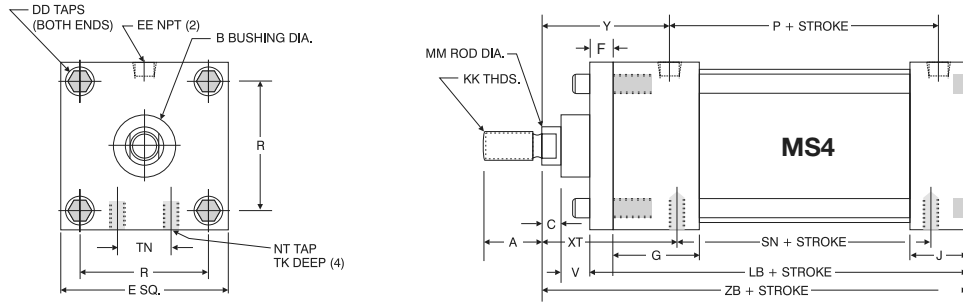
FM Series MS4 Flush Mount Dimensions
